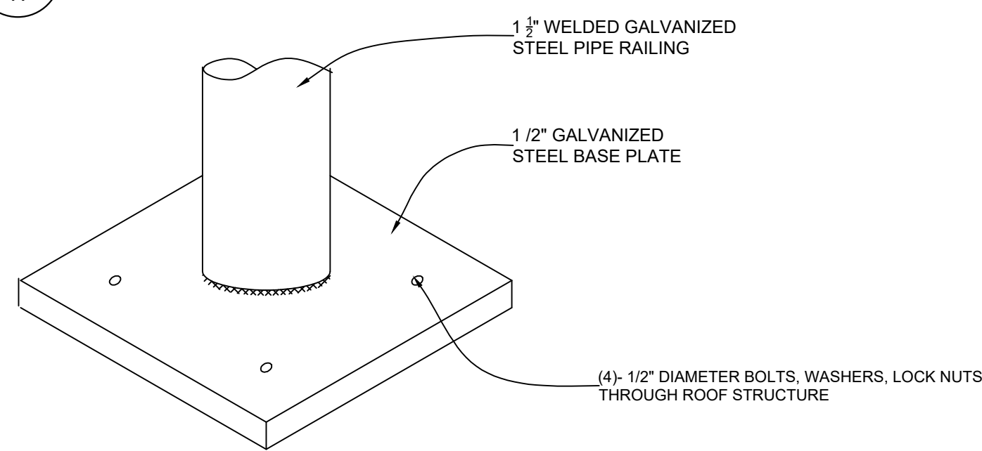
8 RAILING DETAIL 17 NOT TO SCALE
