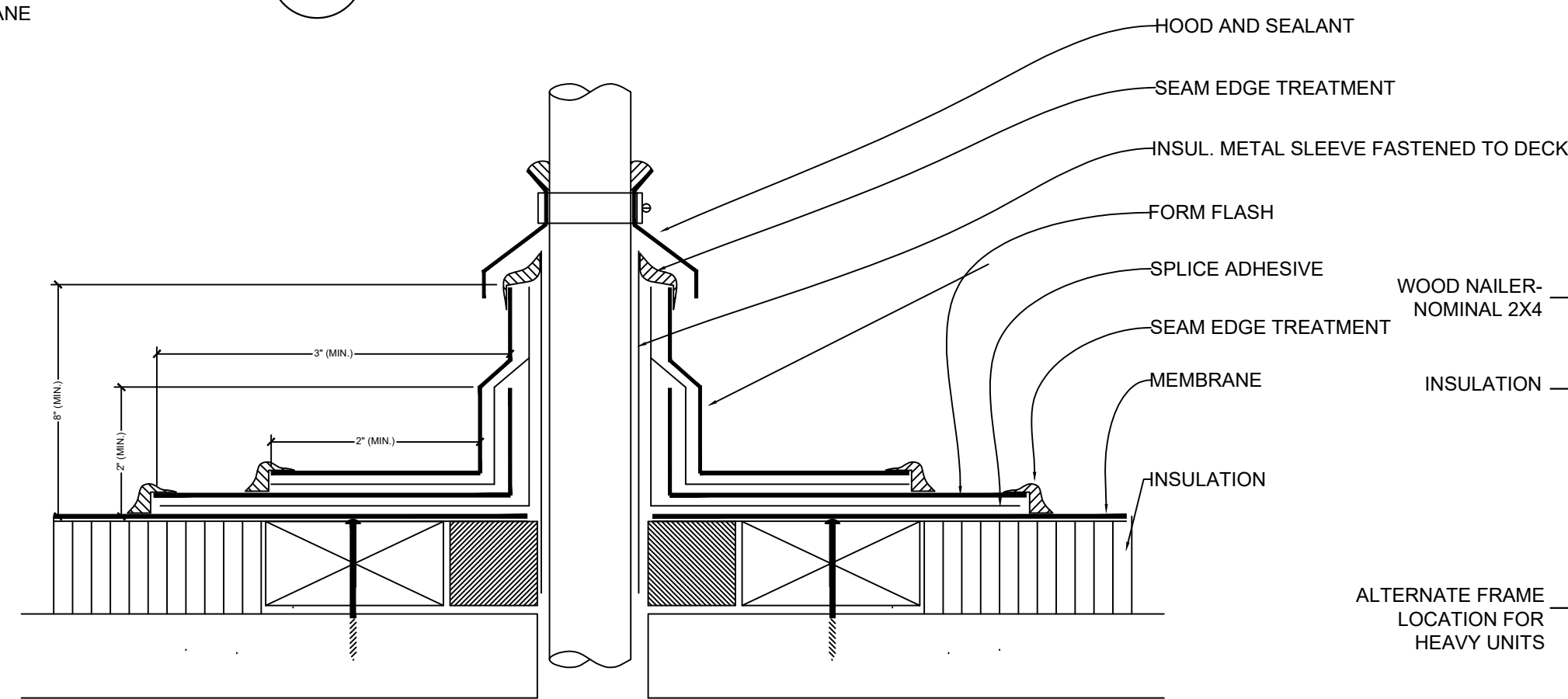
6 HOT STACK FLASHING 17 NOT TO SCALE
